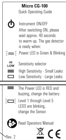
Correct Operating Decal On Back of Gas Sniffer
